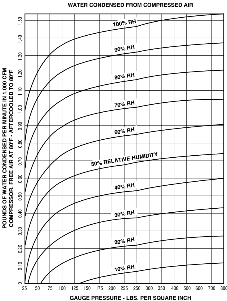
Chart LD-6. Water Condensed From Compressed Air
