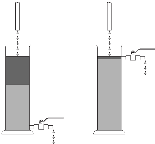
Figure LD-4. If a beaker collecting oil and water is drained from the bottom at the same rate that oil and water enter, it will eventually fill entirely with oil because oil floats on water.
