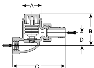
Figure 33-2. TS-2 Trap Straight Type
