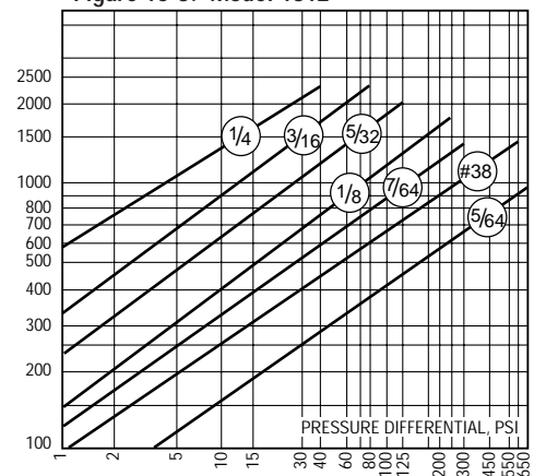
Figure 16-3. Model 1812
