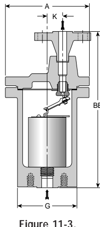
Figure 11-3. Series 300 FW - 400 FW Traps
