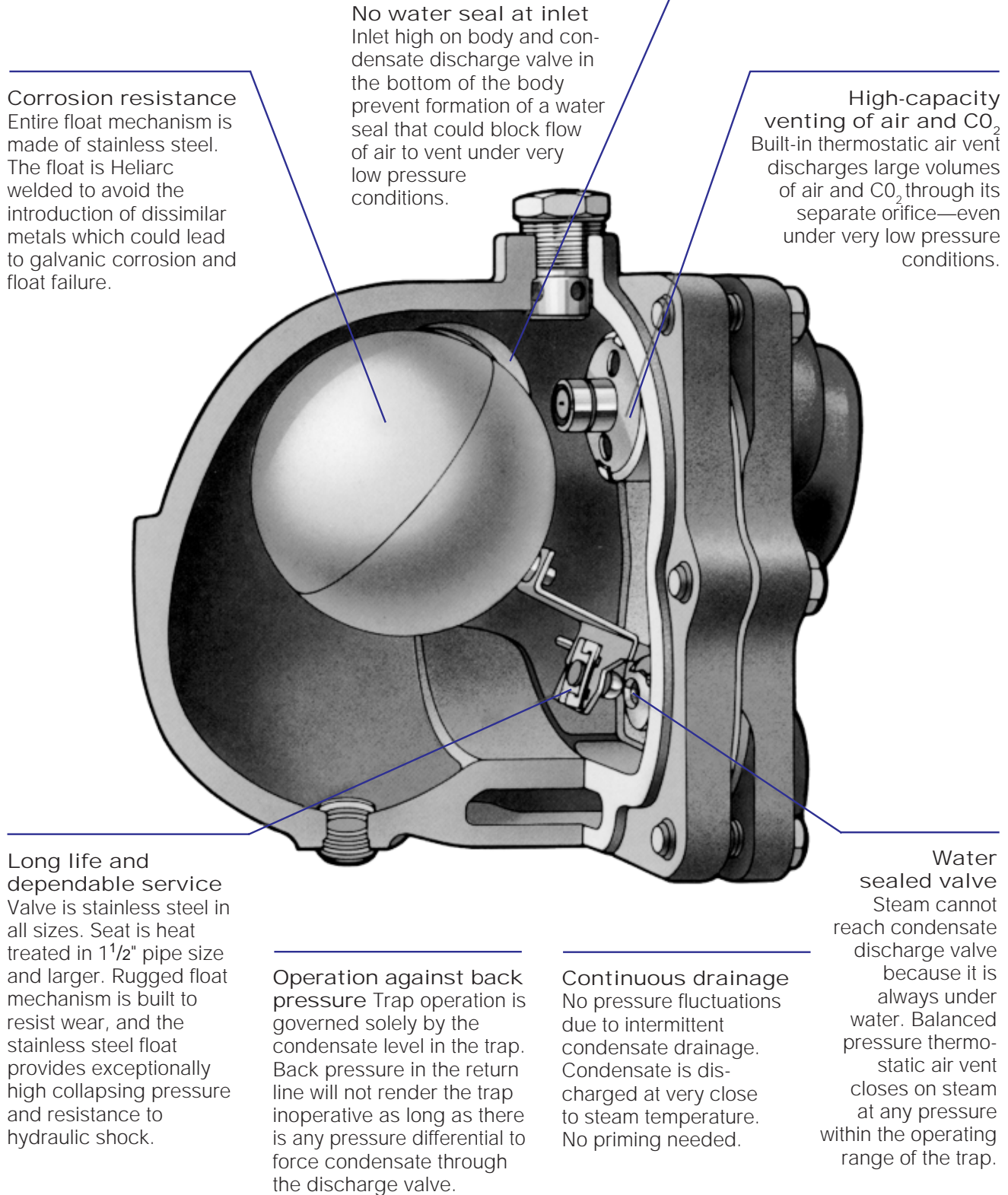
Figure 25-1. Armstrong F&T Design
