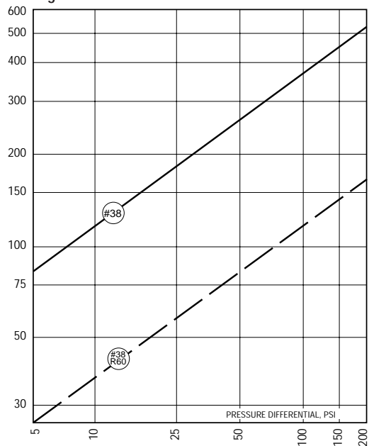
Figure 14-1. Model 2010
