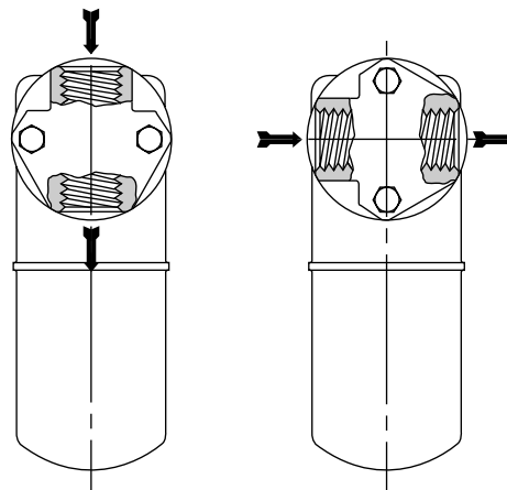
Figure 15-2. Model 2011 Trap
