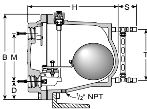
Figure 29-2. Series L and LS, F&T shown
