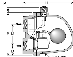
Figure 29-7. Series K, F&T shown
