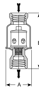
Figure 32-1. TTF-1 Trap
