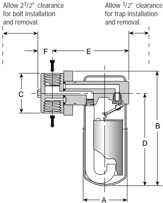
Figure 15-1. Model 2011 Trap
