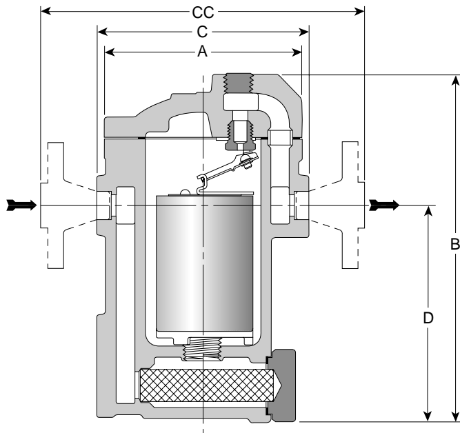
Figure 21-1. Series 980 Cast Steel Traps
