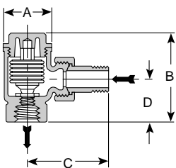
Figure 33-1. TS-2 Trap Angle Type
