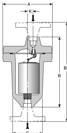
Figure 11-4. Model 411 Trap
