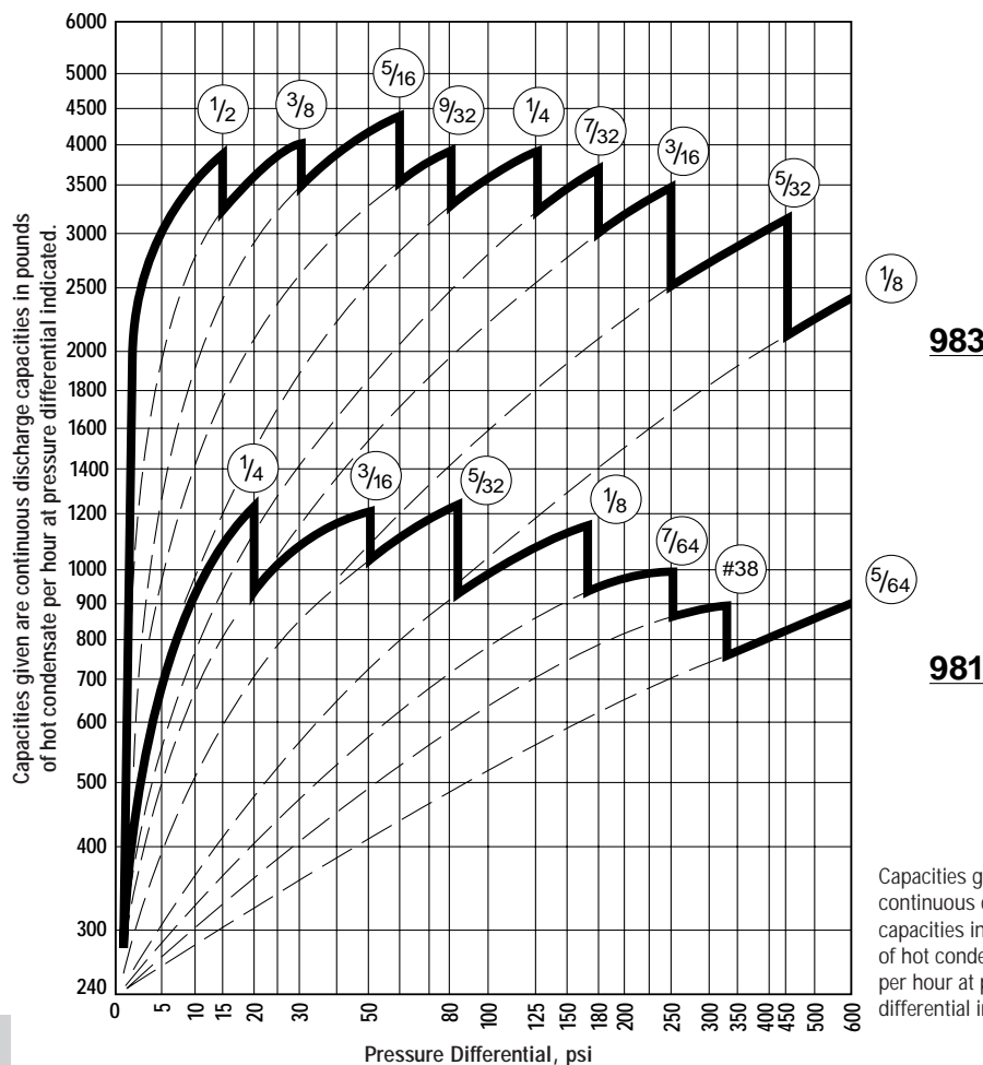
Chart 20-1. Series 980 Traps
