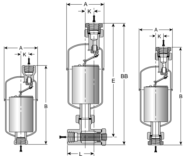
Figure 19-1. Series 1010 Traps
