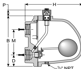
Figure 29-6. Series J, F&T shown
