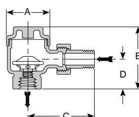
Figure 33-3. TS-3 Trap Angle Type
