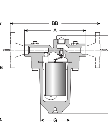
Figure 11-5. Model 421 Trap
