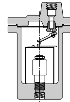
Figure 11-1. Series 300 - 400 Traps with internal check valve
