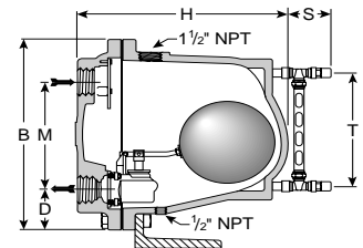
Figure 29-4. Series M and MS, LD shown
