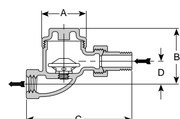
Figure 33-4. TS-3 Trap Straight Type
