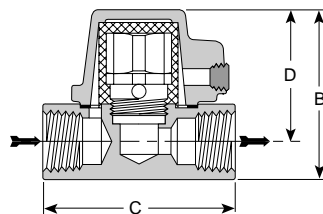
Figure 34-2. Series CD-60 Traps
