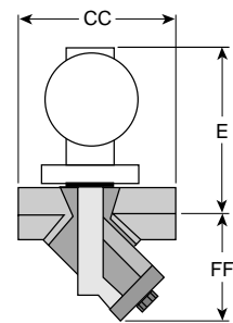
Figure 15-3. Model 2011 with 2010 IS Connector.
