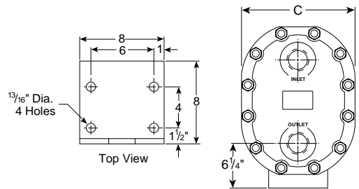
Figure 29-1. LS and MS Floor Mounting Bracket
