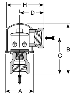
Figure 32-2. TTF-1R Trap
