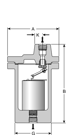
Figure 11-2. Series 300 - 400 Traps
