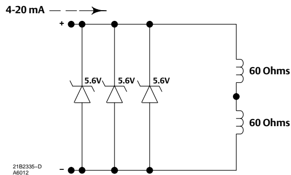
Figure 2. Equivalent Circuit
