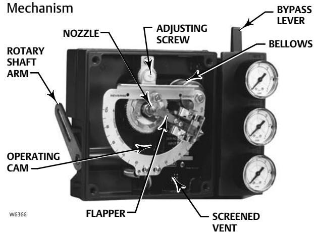
Figure 3. Fisher 3582 Pneumatic Valve Positioner Mechanism
