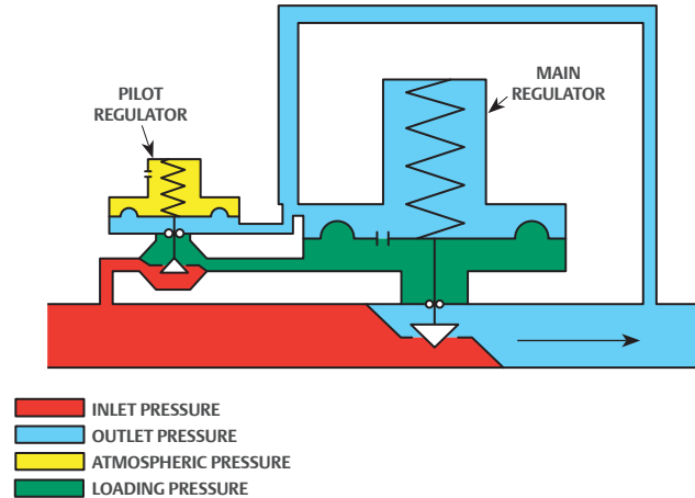
Figure 2. Pilot-Operated Regulator
