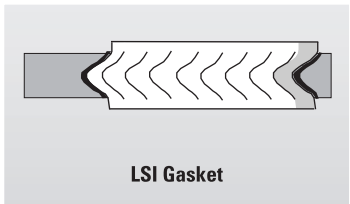
Traditional Spiral Wound Gasket with Inner Ring
