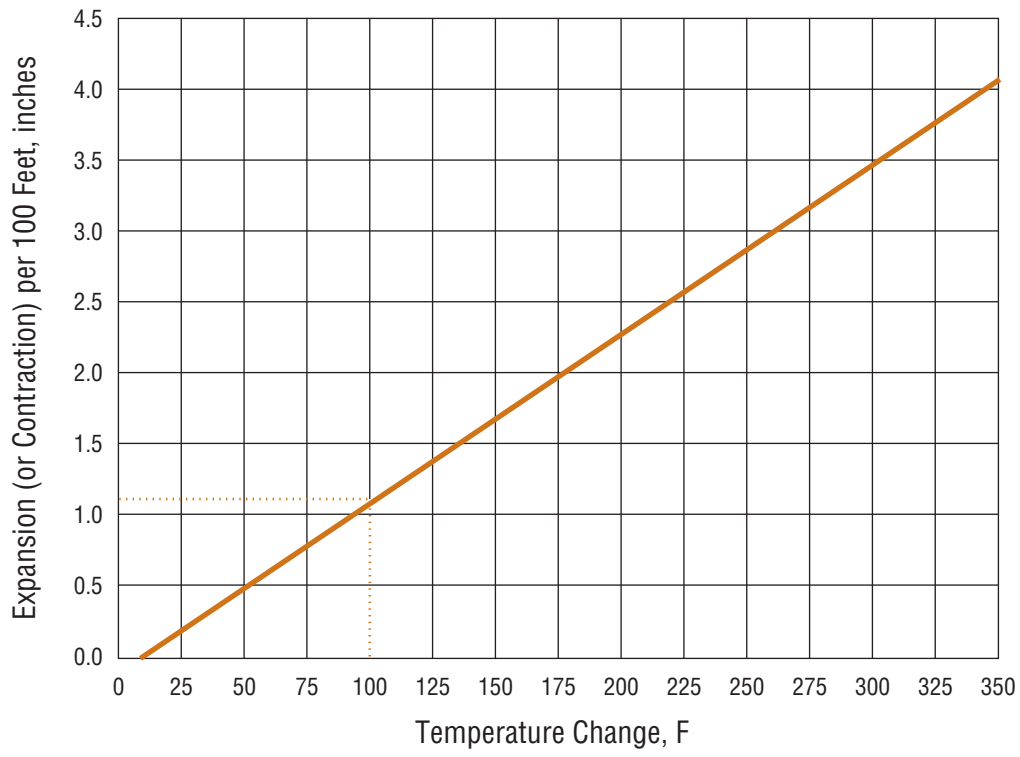
FIGURE 3. Expansion vs. Temperature Change for Copper Tube
