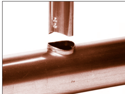
FIGURE 87: Aligning the dimples with the run of the tube
