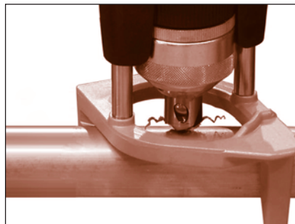
FIGURE 80: Positioning the drill tip and ensuring a snug fit of the support legs
