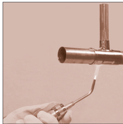
FIGURE 23: Preheating fitting
