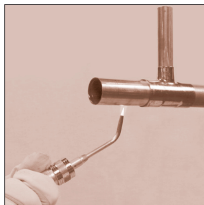
FIGURE 22: Preheating tube
