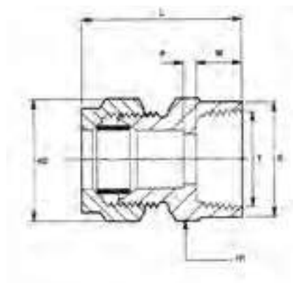
Female Stud Coupling BSPT-Metric
