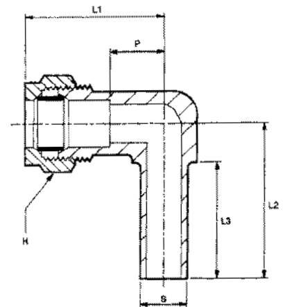
Standpipe Elbow-Imperial
