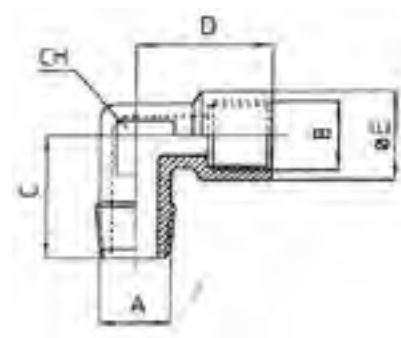
Elbow Male BSPT -Female BSPP
