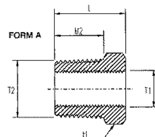
Male BSPT To Female BSPP Adaptor-Form A
